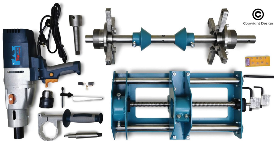
Advance Line Boring Kit
