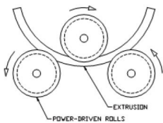
3 ROLL BENDING
