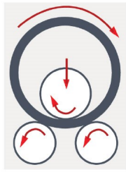
3 ROLL BENDING
