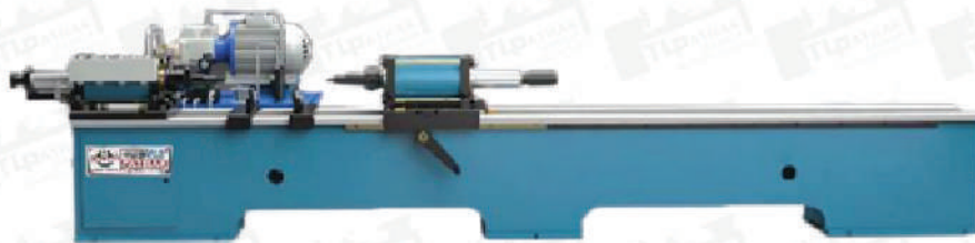
Bearing and Dust Cap Fitting Machine
