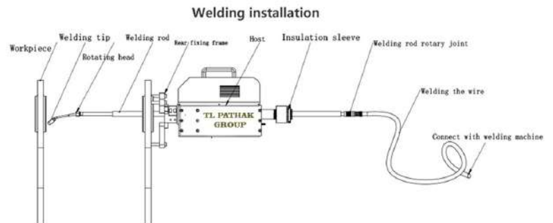
Dioxide Welding Machine Working Component Set
