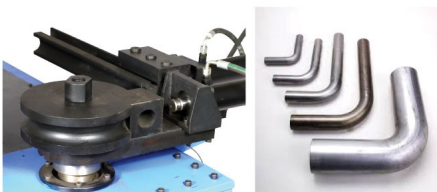
Automatic Hydraulic Pipe Bending Machine
